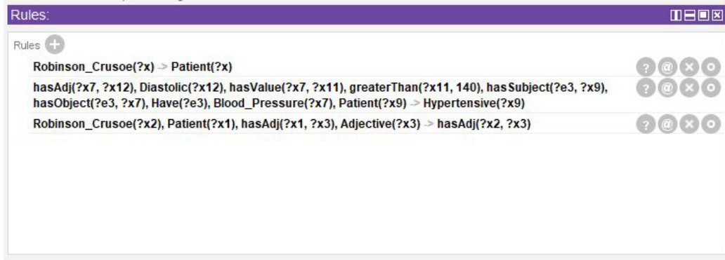
Figure 4: The LODO rules of the case-study
